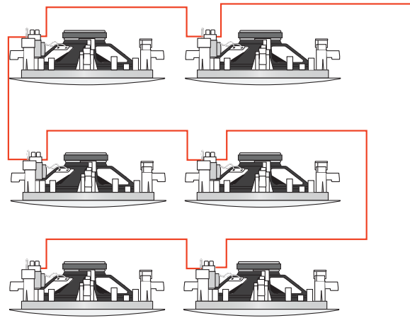
SPEAKER CIRCUIT
